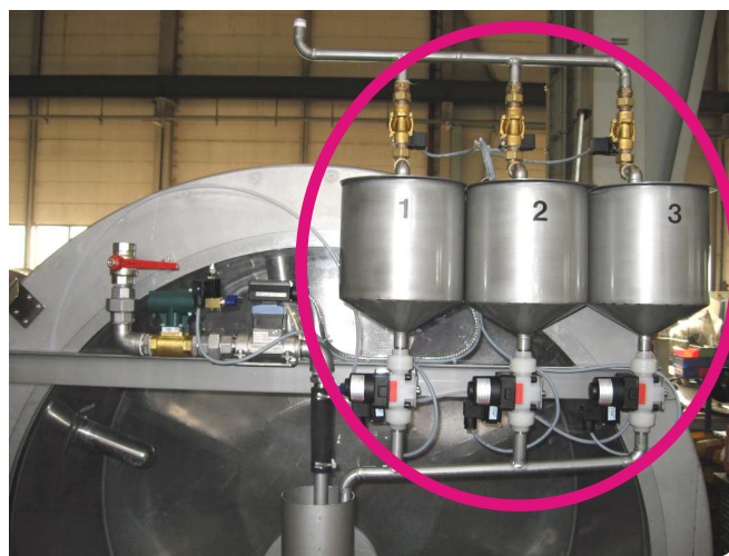
Chemical tank with automatic dosing
